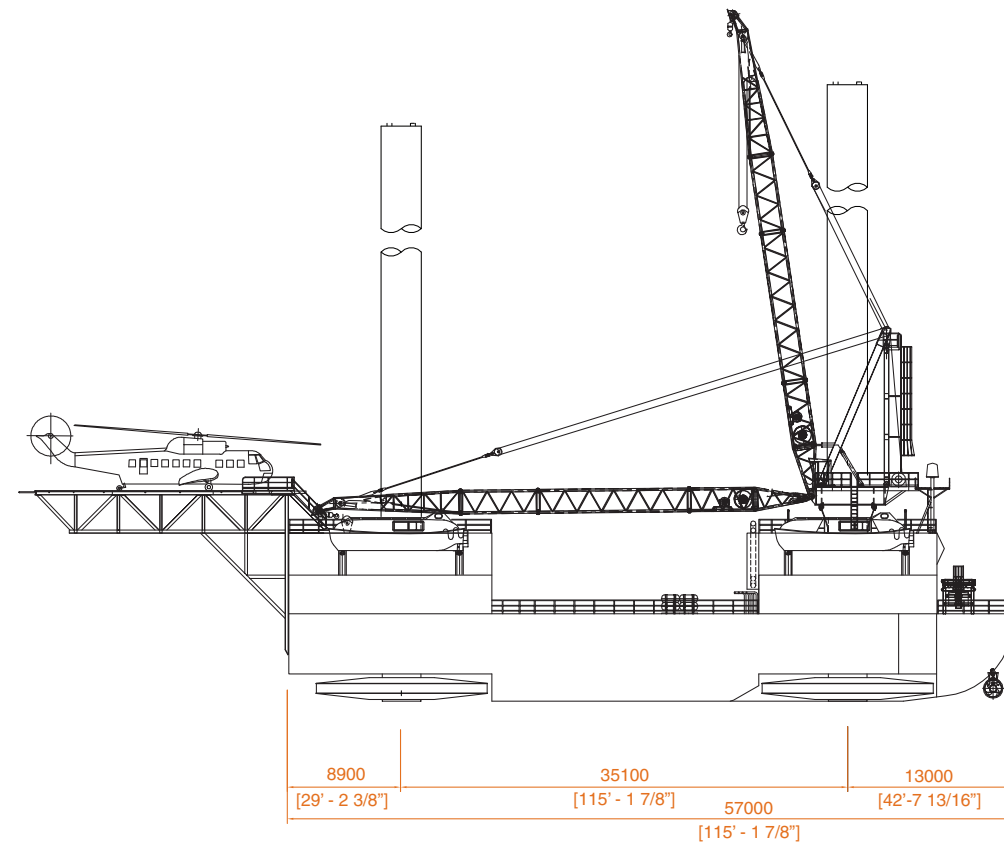
OUTBOARD PROFILE
