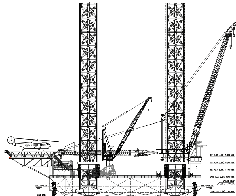
OUTBOARD PROFILE
